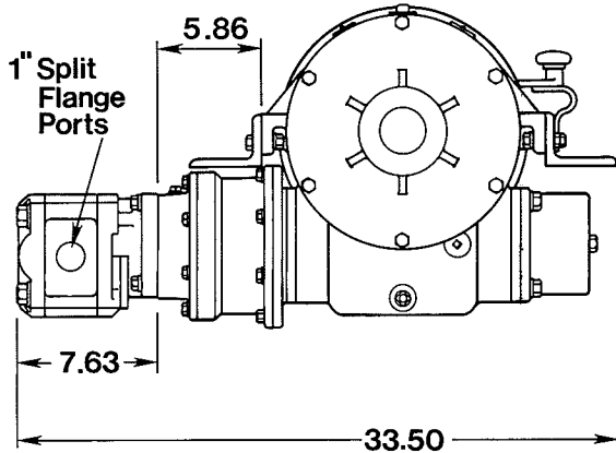
AHSU12P Dimensional
