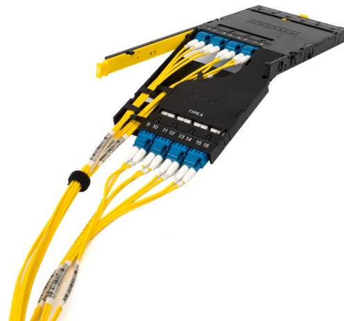
MPO Pivot Module in the Access Position
